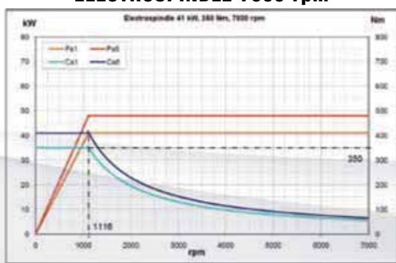
ELECTROSPINDLE 7000 rpm
