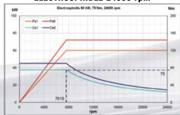
ELECTROSPINDLE 24000 rpm
