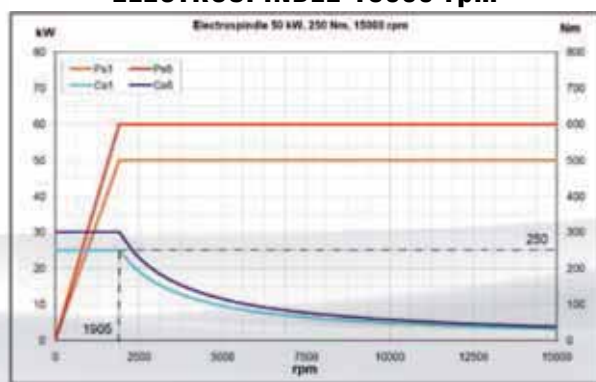
ELECTROSPINDLE 15000 rpm
